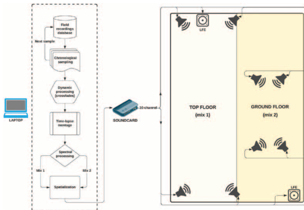
Fig. 4. Time-lapse algorithm routine and audio setup for the 10-channel sound installation at the De Todas las Aguas del Mundo museum in Valdivia. (© Felipe Otondo)
