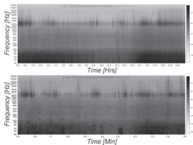
Fig. 2. Comparison between spectrograms of 24-hour continuous recording (top) and 9-minute generated time-lapse montage audio file (bottom). (© Felipe Otondo)
